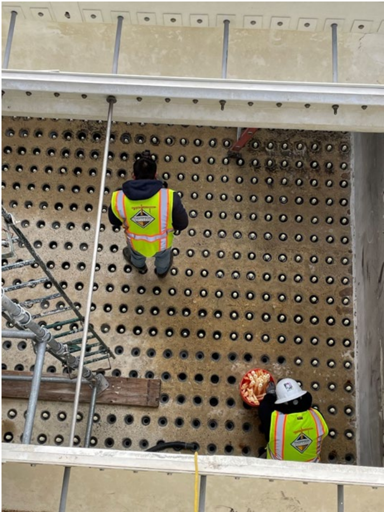
Replacement of Underdrain Nozzles and Domes
