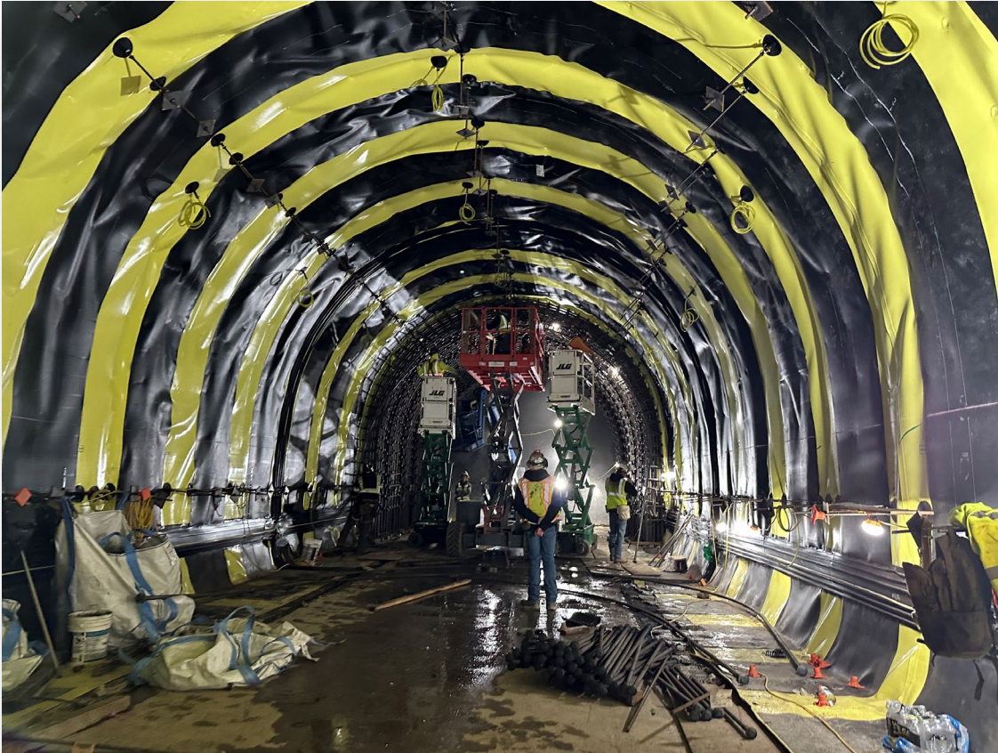
January 2025 Waterproof membrane inside the tunnel
