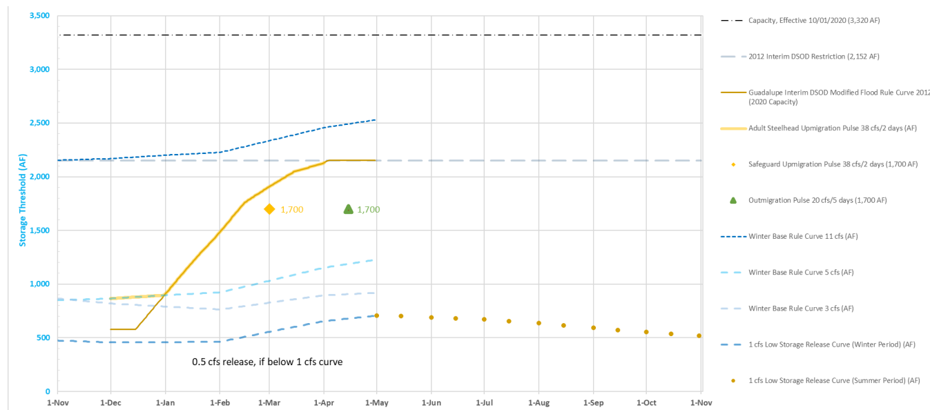
Figure 3. Guadalupe Reservoir FAHCE-plus Reoperation Rule Curves
