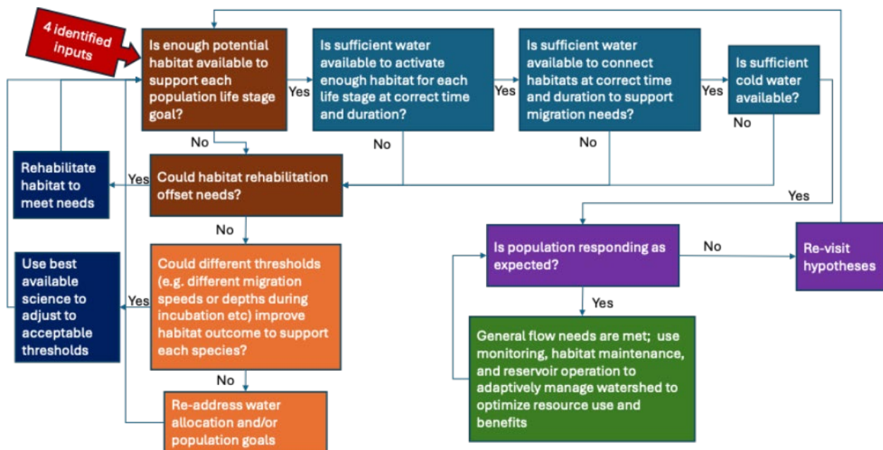
Figure 11. Iterative Process
