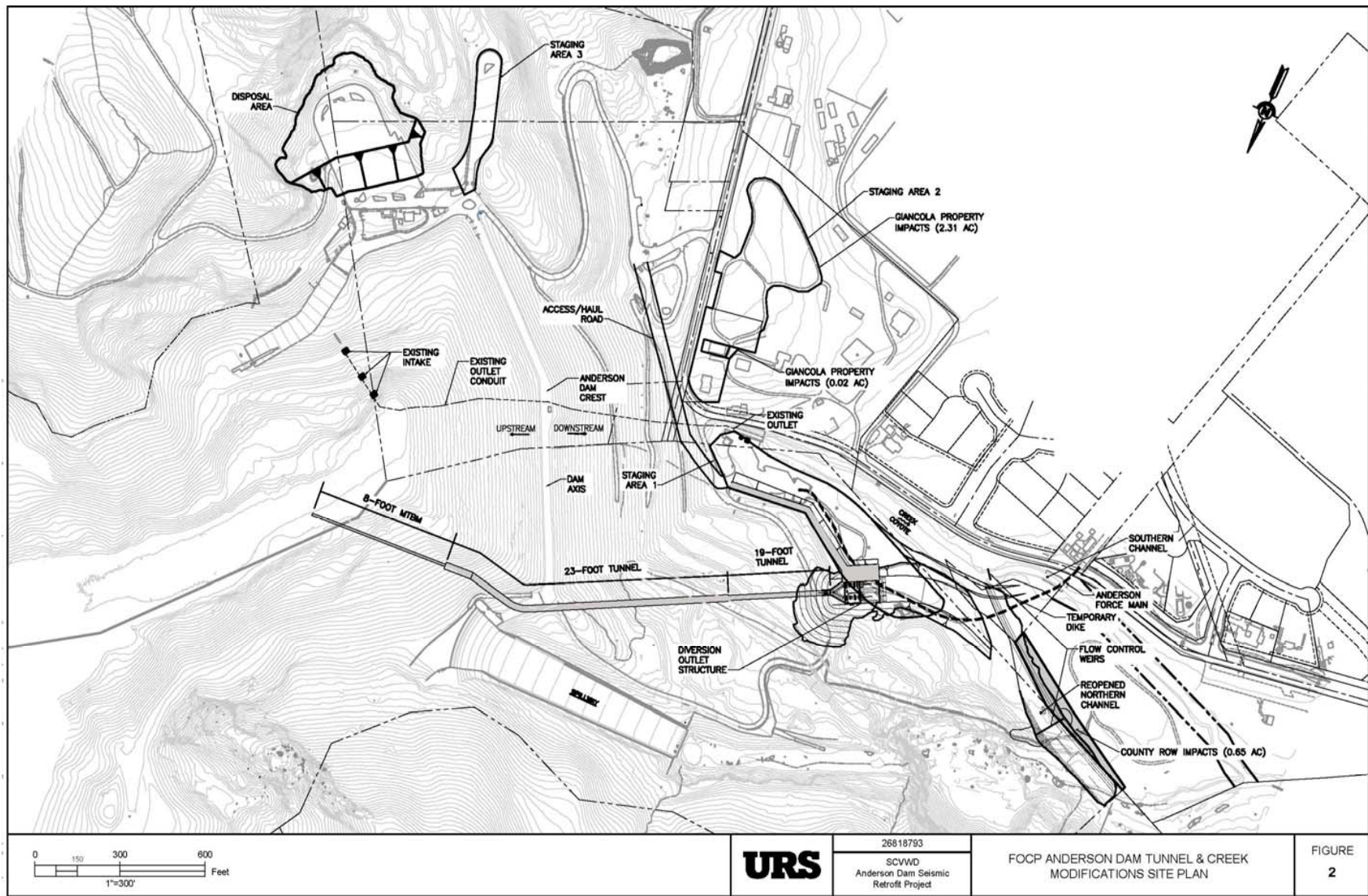
Figure 2. FOCP Anderson Dam Tunnel Project and Creek Modifications Site Plan
