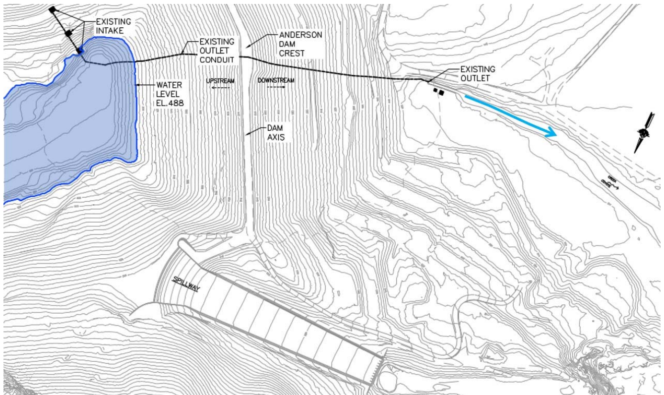
Figure 4: Reservoir Water Surface Elevations and Flow Paths for Drawdown and ADTP Years 1 through Years 3
