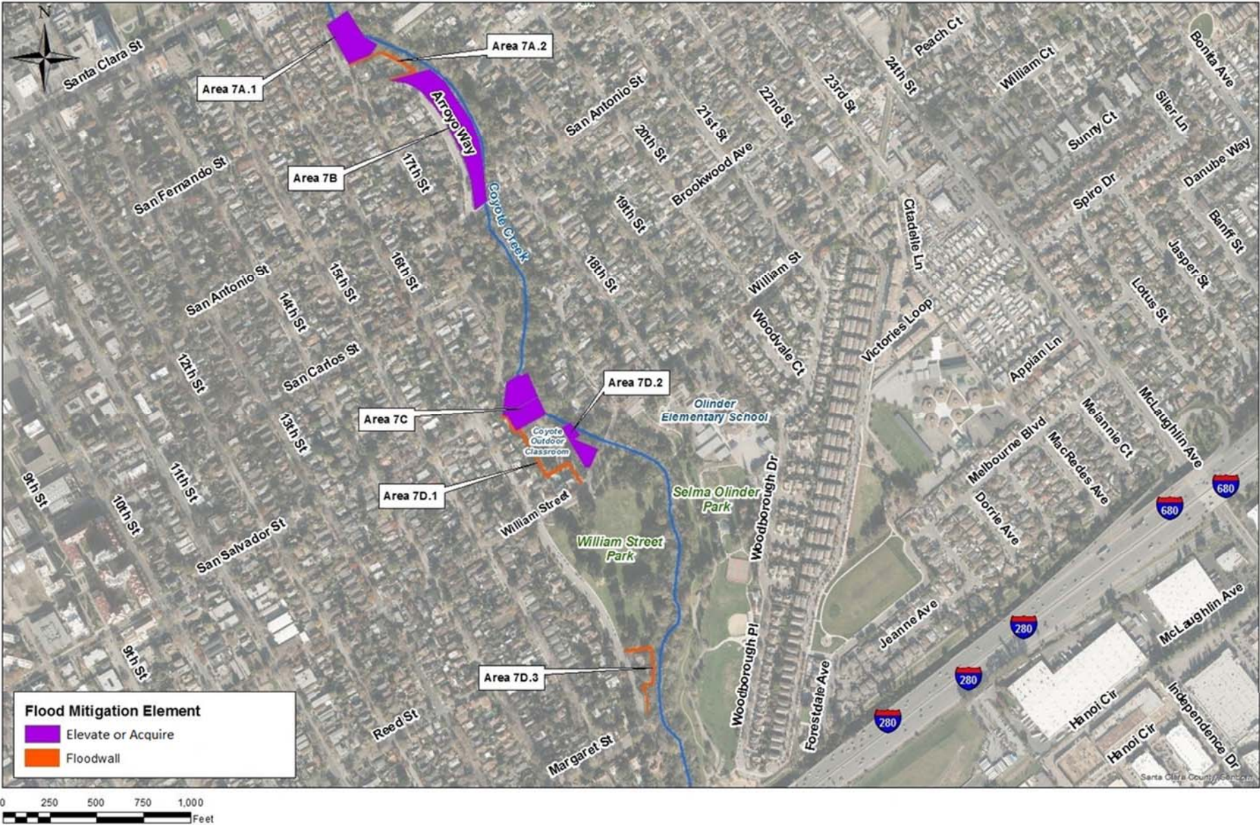
Figure 9c. FOCF Coyote Creek Flood Management Measures Site Plan (Reach 7)
